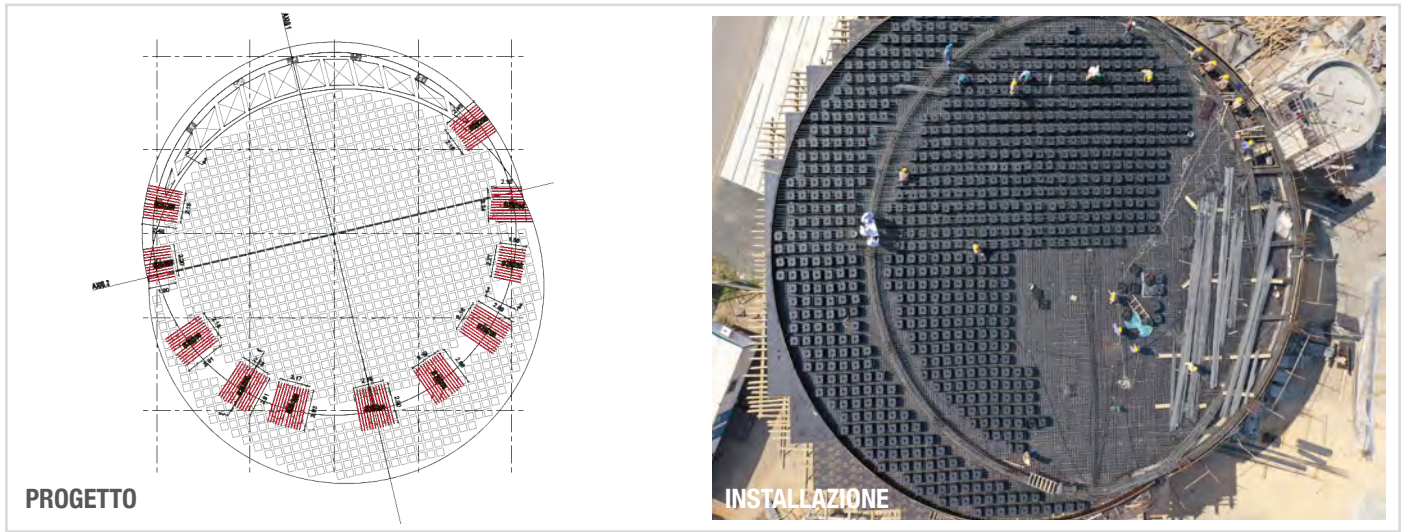
Moschea Mahboob Bin Al Ruhal, Oman
